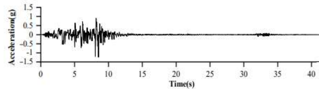
Figure 2. Seismic acceleration time history curve
