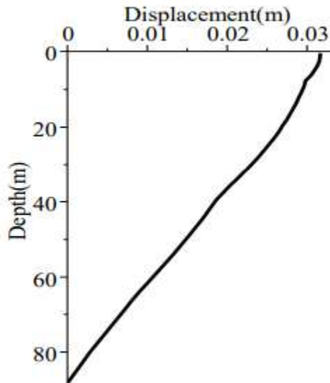
Figure 4. Maximum relative displacement of soil
