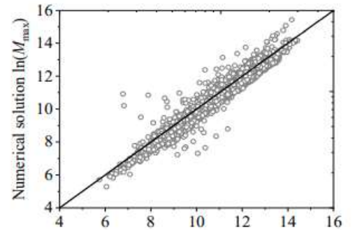
Predicted value of deterministic model \ln(M_{max})
