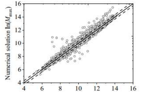
Predicted value of probabilistic model \ln(M_{max})
