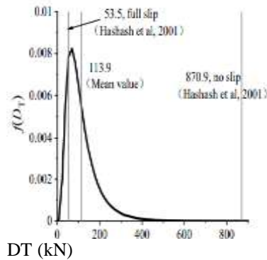
(b) Axial force Figure 9. Demand probabilistic density functions
